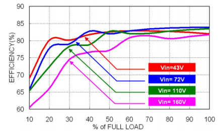
43RDL06-110S05W Efficiency vs. Output Load
