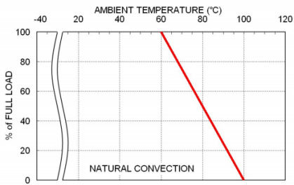
43RDL06-110S05W Derating Curve
