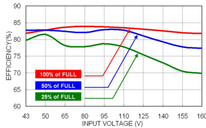
43RDL06-110S05W Efficiency vs. Input Voltage
